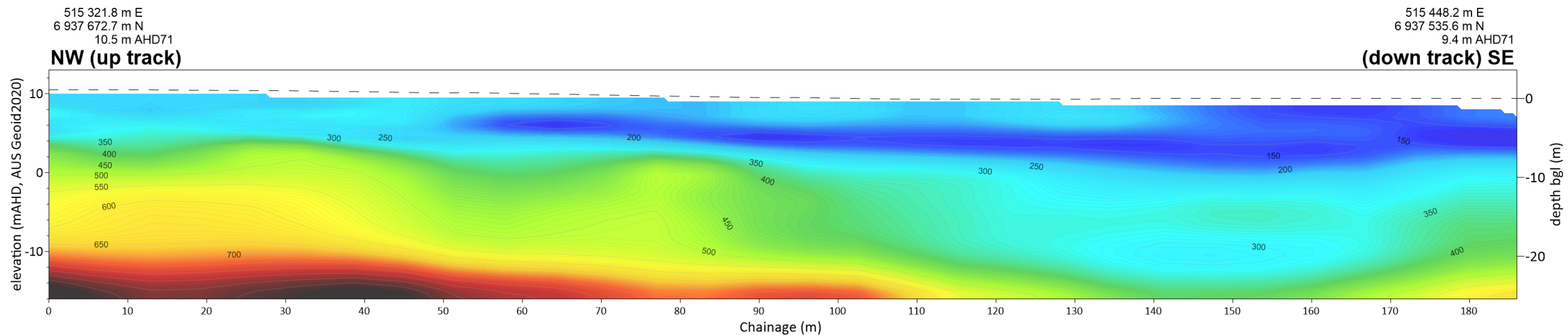
Seismic Line MASW AU-GP 164-1
